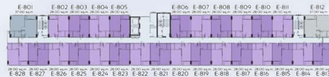
8 th Floor plan
