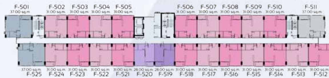
5 th Floor plan
