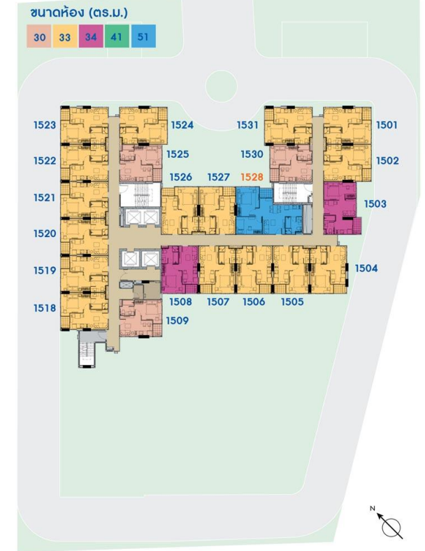
15 th floor
